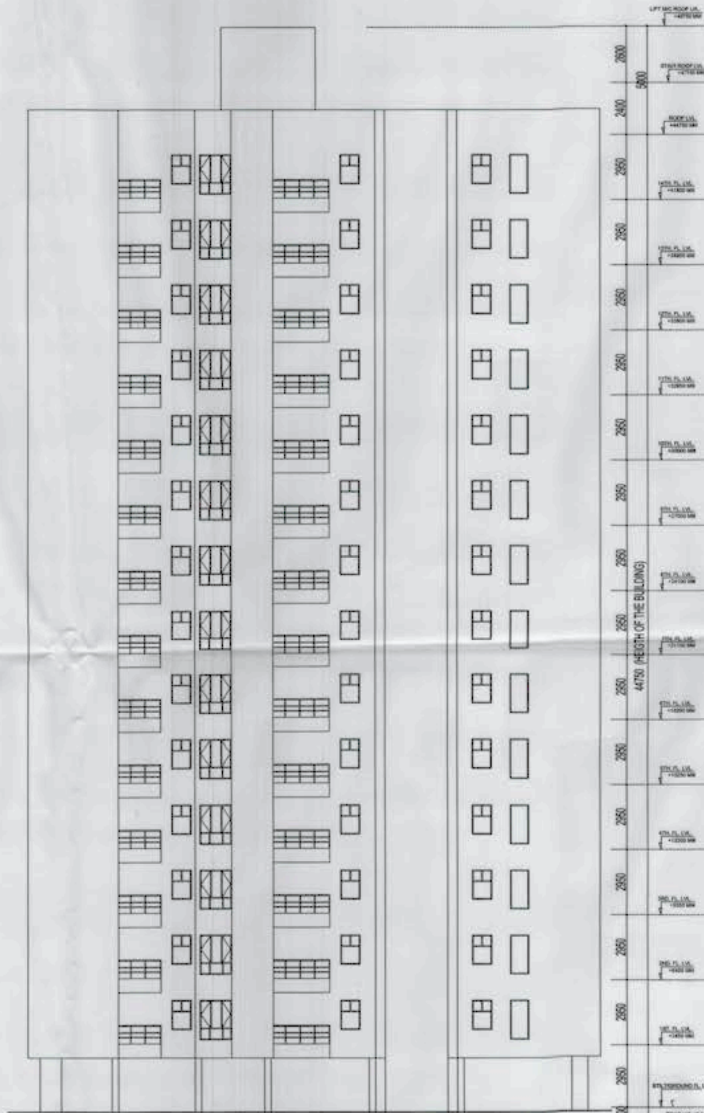
LEFT SIDE ELEVATION
